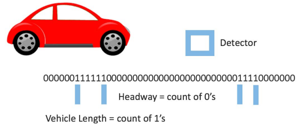
Fig. 1. Scheme of a traffic detector. Source: TfL.
