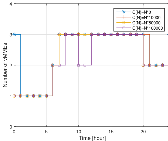
Fig. 13. N_{\text{opt}} for different costs C(N) , during January 23, 2015.
